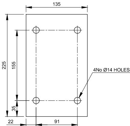
TPL-C-2 - 10mm THICK Scale 1:5
