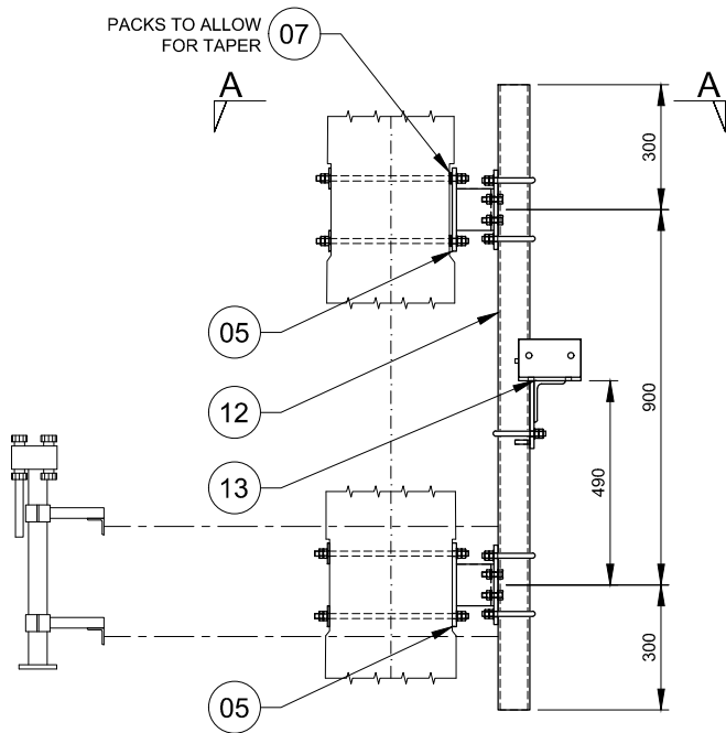
DETAIL H - Rx ANTENNA MOUNT Scale 1:20
