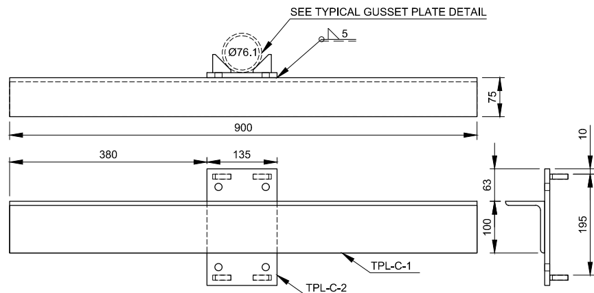
TPL-C - UA100x75x8 Scale 1:10
