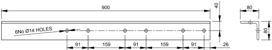
TPL-A-1 - EA 80x80x8 Scale 1:10
