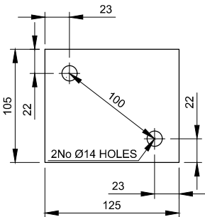
TPL-1 - 10mm THICK Scale 1:5
