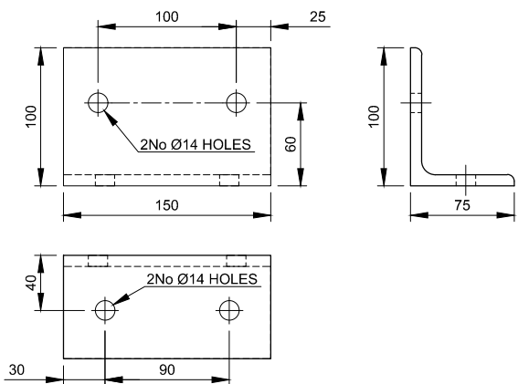
TPL-C-3 - UA100x75x8 Scale 1:5
