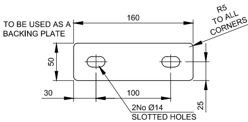
TPB-B-4 - 5mm THICK Scale 1:5
