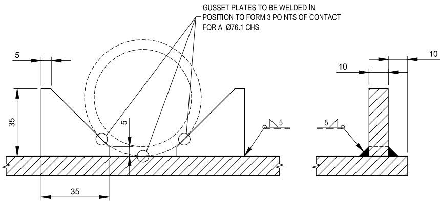
TYPICAL GUSSET PLATE DETAIL Scale 1:2
