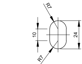
SLOTTED HOLE DETAIL Scale 1:2
