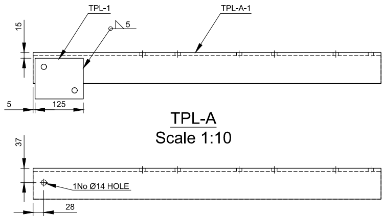
TPL-A-1 - EA 80x80x8 Scale 1:10
