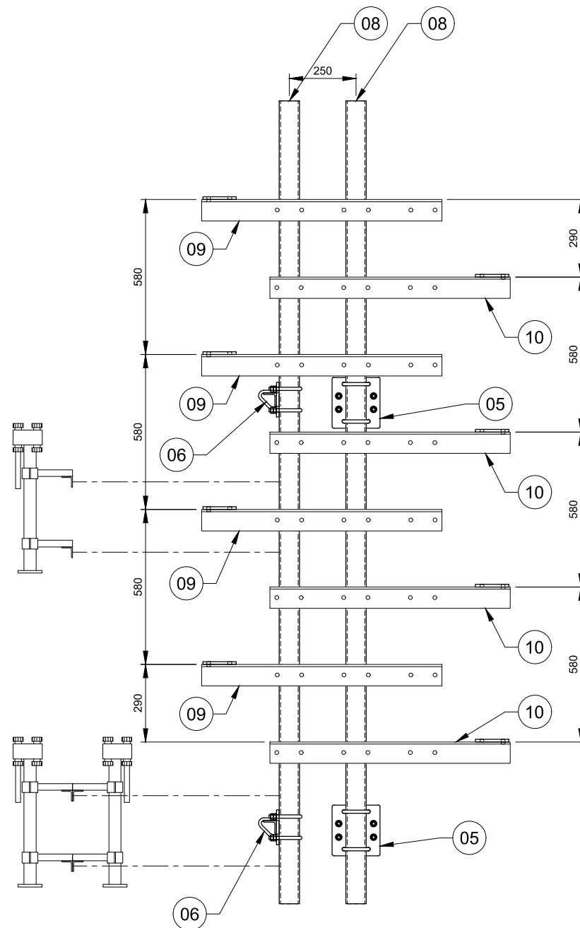
SECTION B-B Scale 1:20
