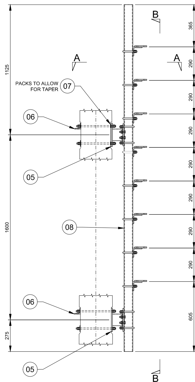
DETAIL G - Tx ANTENNA MOUNT Scale 1:20
